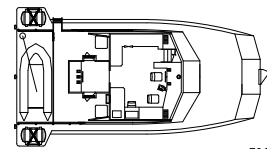
FOCSLE DECK
