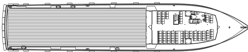
MAIN DECK
