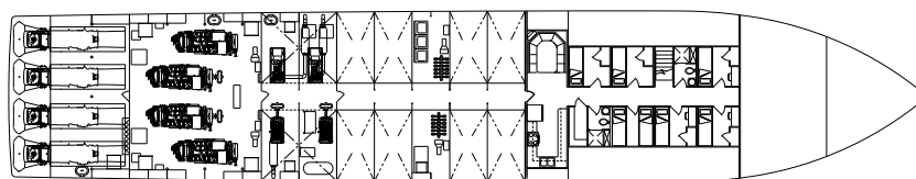
BELOW DECK
