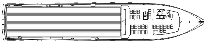
MAIN DECK
