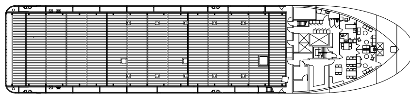
MAIN DECK
